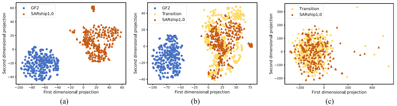
Fig. 10. Visualized t-SNE results of feature distributions, where each blue dot denotes one image feature of the optical GF2ship dataset, each red triangle denotes one image feature of the SARship dataset, and each orange blot denotes one image feature of the transition domain. All the features are extracted by the last convolutions of VGG16. (a) Original results of the optical domain and SAR domain. (b) Result after pixel-level adaptation. (c) Result after feature-level adaptation.
