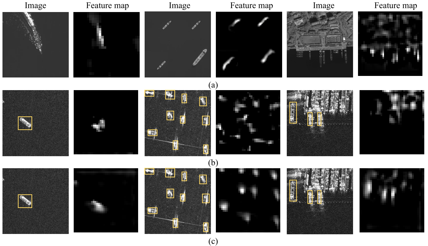
Fig. 14. Visualization of deep feature representation. (a) Optical GF2ship images and corresponding feature maps extracted by the supervised faster R-CNN trained on the GF2ship dataset. (b) SAR images and the corresponding feature maps directly extracted by the supervised faster R-CNN trained on the GF2ship dataset without adaptation. (c) SAR images and the corresponding feature maps extracted by our UDA faster R-CNN model. SAR images in (b) and (c) are same, and yellow rectangles represent ship targets in SAR images.
