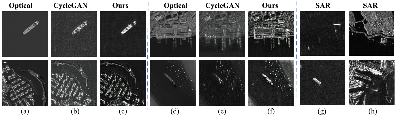
Fig. 8. Visualized generation results of OSGAN and comparison CycleGAN. (a) and (d) Original optical images, (b) and (e) corresponding generation results of CycleGAN, (c) and (f) corresponding generation results of our OSGAN. (g) and (h) Four images of real SAR images in AIR-SARShip-1.0.
