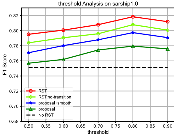
Fig. 12. Ship detection performance with different variants and threshold, and F1-score of our RST reaches the peak when the threshold is 0.8.
