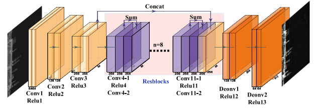
Fig. 4. Architecture of the generator with skip connection.
