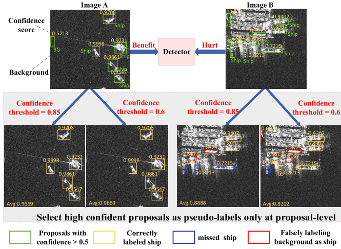
Fig. 5. Selecting proposals as pseudo-labels at the proposal level for two SAR images. For Image A, the correct pseudo-labels are more whether setting a high confidence threshold or a low confidence threshold. For Image B, wrong pseudo-labels are more. When setting a high threshold, some ships will be treated as backgrounds; when setting a low threshold, some backgrounds will be treated as ships.
