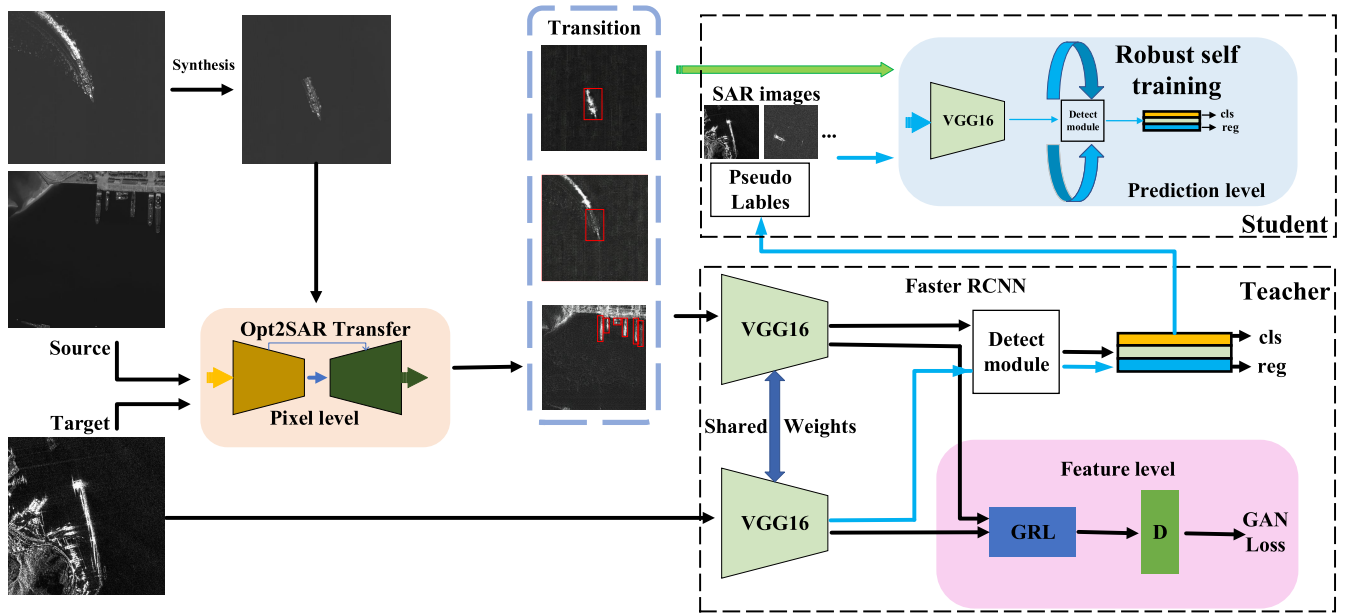
Fig. 2. Architecture of the unsupervised cross-domain adaptation framework based on progressive transfer for SAR ship detection. At the pixel level, Opt2SAR transfer transfers the source and synthesis images to transition images. At the feature level, the parameters of VGG16 are shared between two domains and GAN loss is used to learn the domain-invariant feature representation. The blue lines represent the flow of pseudo-labels' generation. At the prediction level, we treat the detector obtained in the previous stage as a teacher model and generate the pseudo-labels by testing on the unlabeled training target SAR images.
